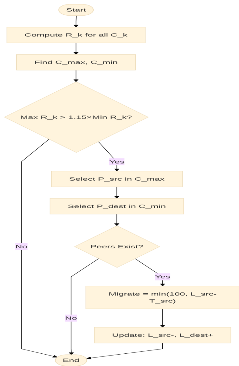
Figure 6: Inter-Region Load Balancing Flowchart
